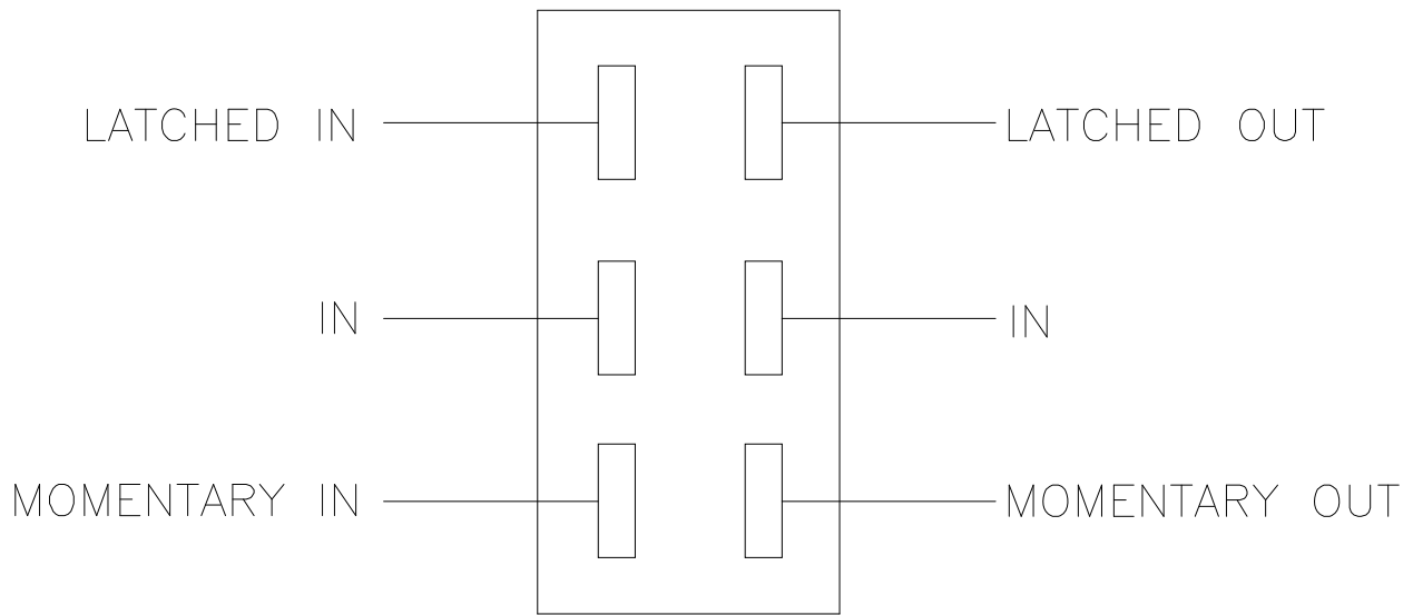
STANDARD DPDT SWITCH (MOMENTARY - LATCHED)
